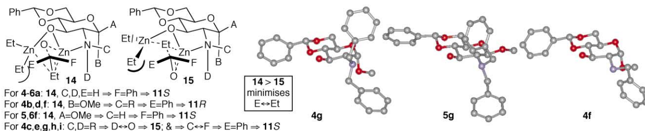
Fig. 1 Proposed model consistent with mode of asymmetric addition 8 → 11 and corresponding X-ray structures. § of 4g , 5g , 4f .
